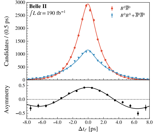
FIG. 3. Distribution of \Delta t_\ell in data (points) and the fit model (lines) for opposite-flavor candidate pairs (red) and same-flavor pairs (blue) and their asymmetry (black).
